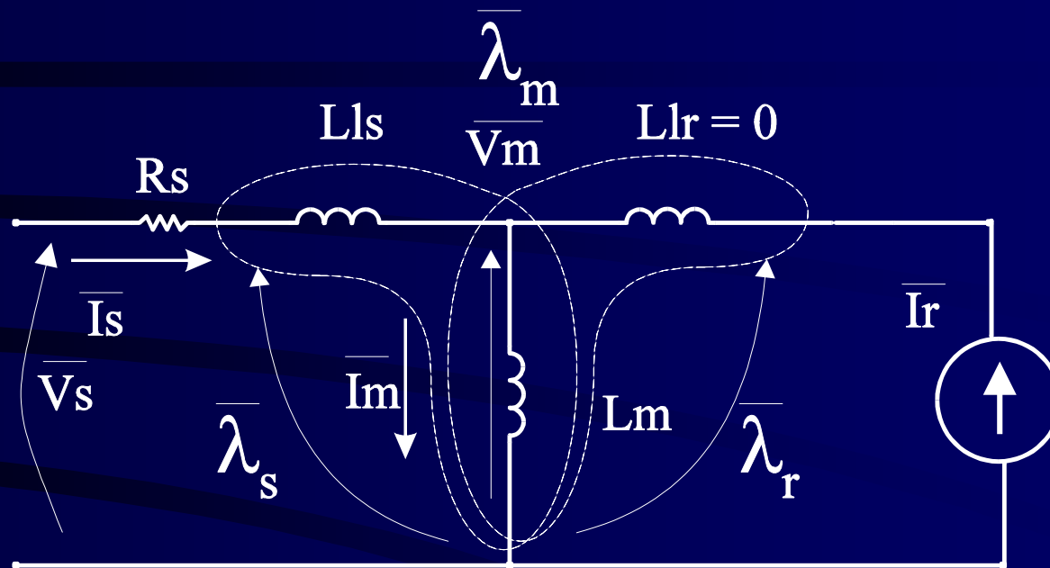
PM Synchronous Motor Model
